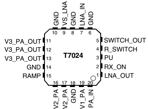
Figure 3. Pinning QFN20
