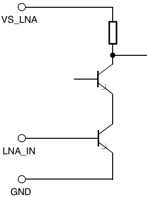
Figure 25. Input Circuit LNA_IN/VS_LNA
