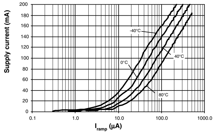
Figure 17. PA (PSSO20): Supply Current versus I_{\text{ramp}} and Temperature
